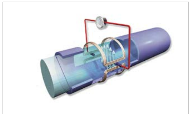
Figure 1. The velocity deflects the standing magnetic field and induces a voltage on the electrodes that is proportional to velocity.
