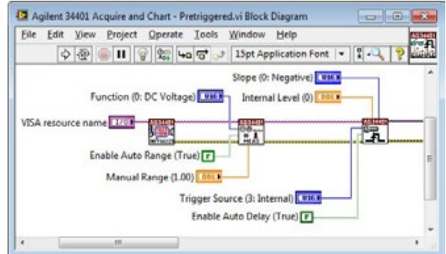
LabVIEW Code
